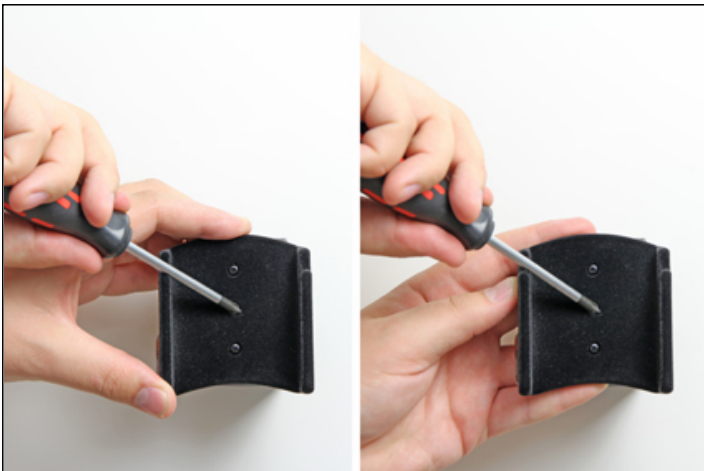
3. Start to thread the center screw into the base plate. When you connect with the nut pull the holder towards you to prevent the nut from spinning around. Continue to tighten the screw firmly. Then loosen the screw slightly for easier angling/rotation of the holder.
