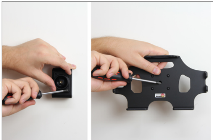
2. Place the base plate over the matching holes in your mounting bracket (demo ProClip mount shown in picture) Attach the base plate by using the self-tapping screws. Note: The machine screws with nuts are for mounts made of metal with large holes. Start to thread the center screw into the base plate. When you connect with the nut pull the holder towards you to prevent the nut from spinning around. Continue to tighten the screw firmly. Then loosen the screw slightly for easier angling/rotation of the holder.
