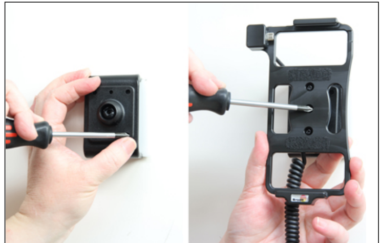
2. Place the Tilt Swivel base plate over the matching holes in your mounting bracket (demo ProClip mount shown in picture) Attach the base plate by using the self-tapping screws. Place the holder onto the base plate. Start to thread the center screw into the base plate. When you connect with the nut pull the holder towards you to prevent the nut from spinning around. Continue to tighten the screw firmly. Then loosen the screw slightly for easier angling/rotation of the holder.
